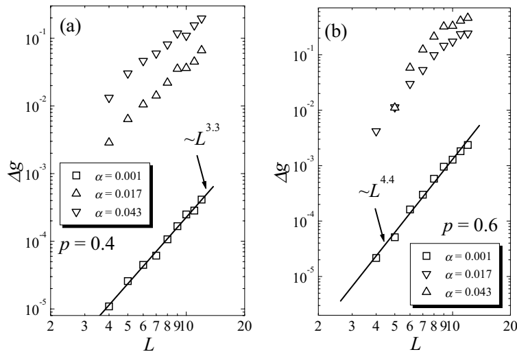
Fig. 2. Magnetoconductance \Delta g versus system size L for different content of metallic phase: (a) p = 0.4 , (b) p = 0.6 . Results for various magnetic fluxes \alpha are shown. Data for \alpha = 0.001 (weak magnetic field) are fitted by the straight line. The slopes of the fitting lines are: 3.3 for p = 0.4 , 4.4 for p = 0.6 .
