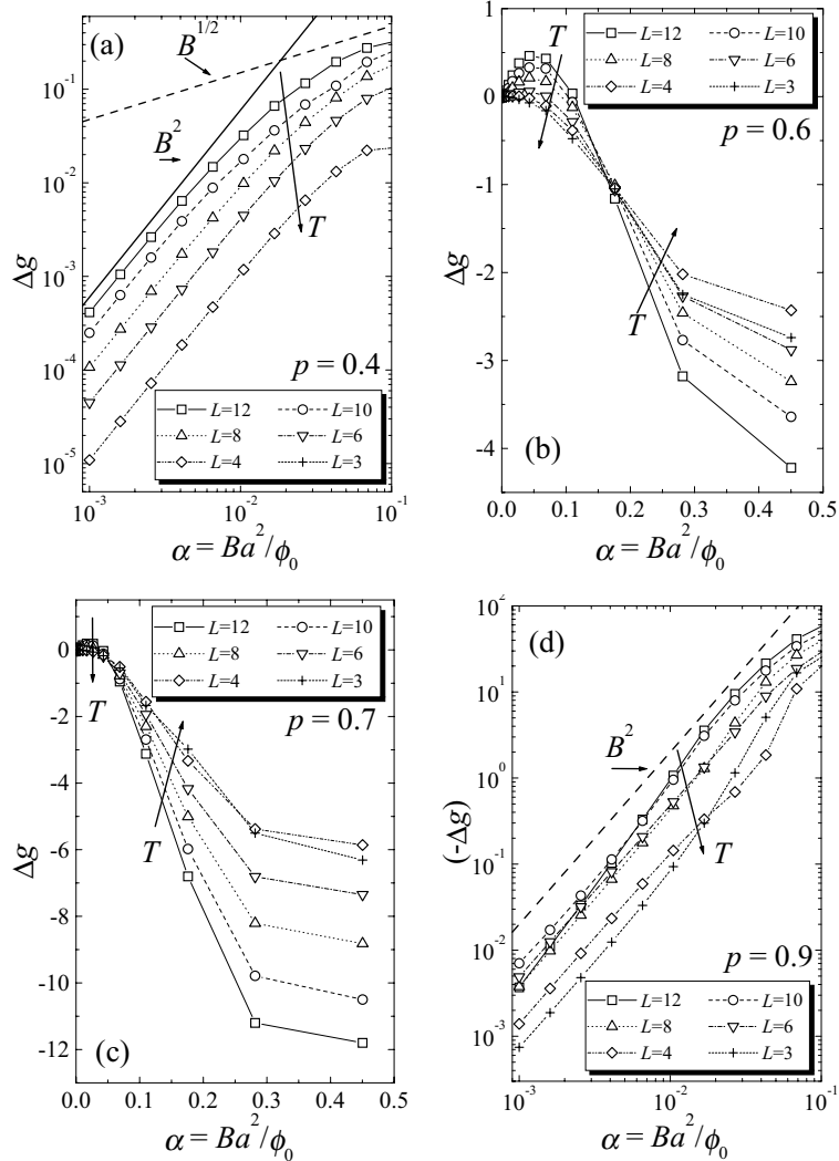
Fig. 1. Magnetoconductance \Delta g versus magnetic flux \alpha for various content of metallic phase: (a) p = 0.4 , (b) p = 0.6 , (c) p = 0.7 , (d) p = 0.9 . Series for different sizes L of the system are shown. Lines marked as being proportional to B^2 and B^{1/2} are included as a reference. Arrows point tendency when temperature T increases. Magnetoconductance is positive for p = 0.4 (Fig. 1(a)) and negative for p = 0.9 (Fig. 1(d)) in studied span of magnetic flux. It changes its sign for intermediate values of concentration p (Figs 1(b) and 1(c)) hence the scales are linear in these cases. Lines connecting points are added to guide an eye.
